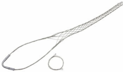
FS050U: Standard Duty, Split Lace, Single Eye, Cable Diameter 0.05 - 0.61 inches, Bale Length 7-in, Mesh Length 11-in, Break Strength 770 lbs.
