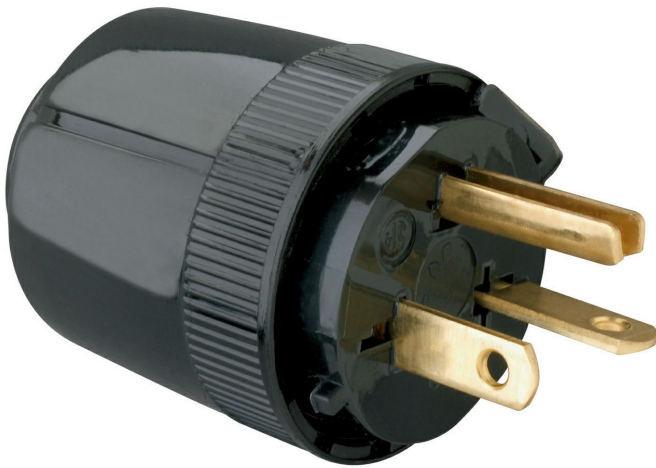
Straight Blade Plug 20A 250V Dead Front
